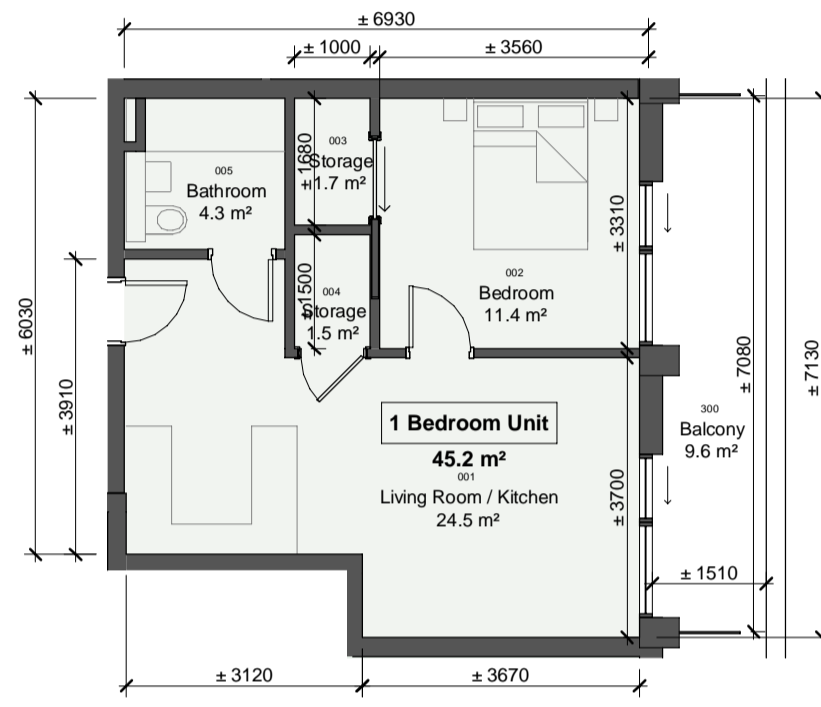
5 Unit Type 1BR-D-1 scale 1 : 100
