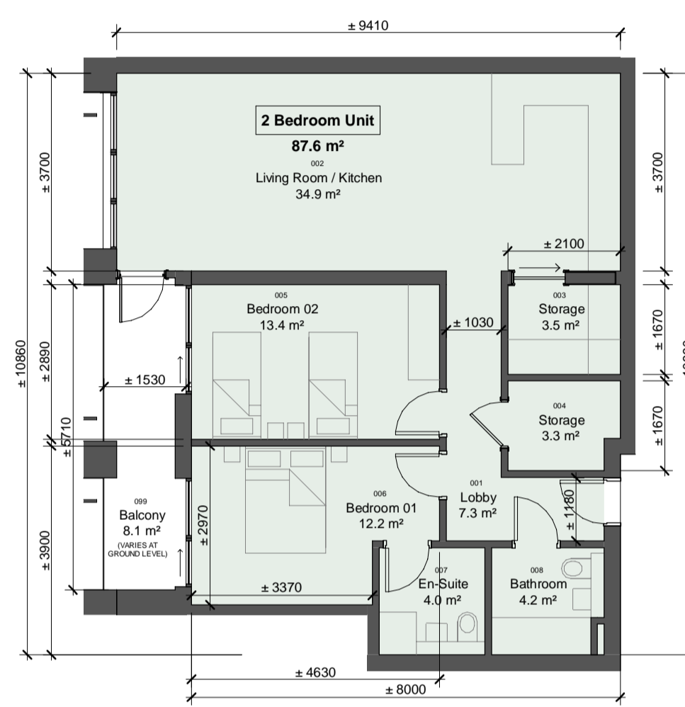
6 Unit Type 2BR-A-1 scale 1 : 100
