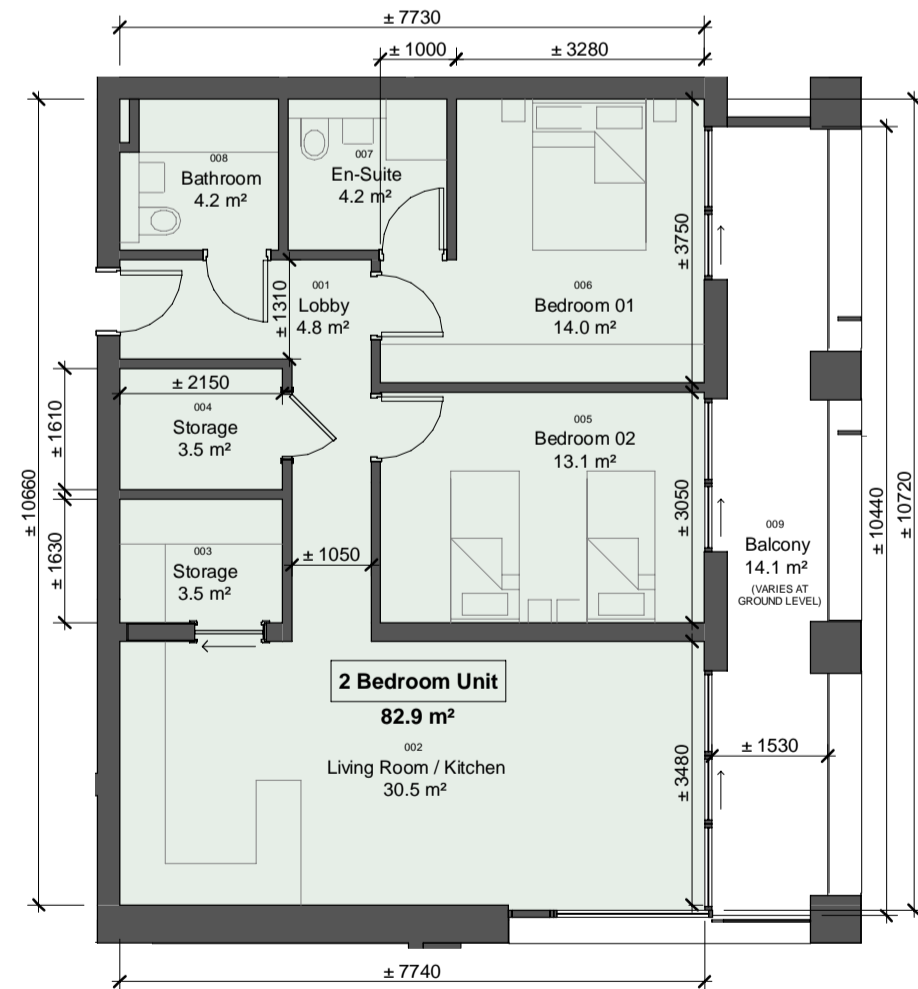
9 Unit Type 2BR-C-1 scale 1 : 100
