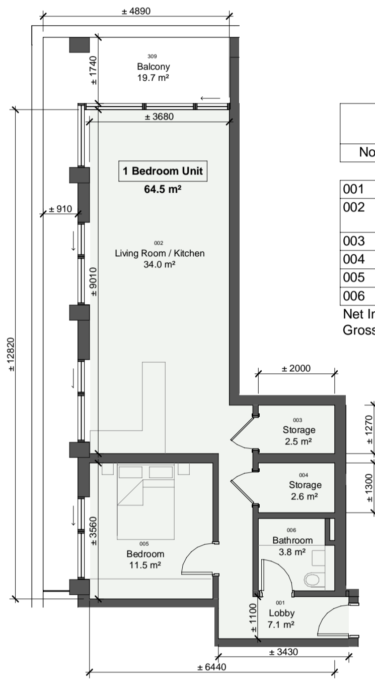
4 Unit Type 1BR-C-1 scale 1 : 100
