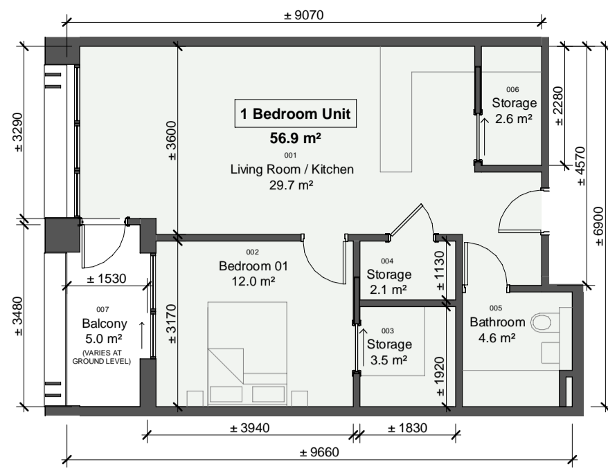
1 Unit Type 1BR-A-1 scale 1 : 100
