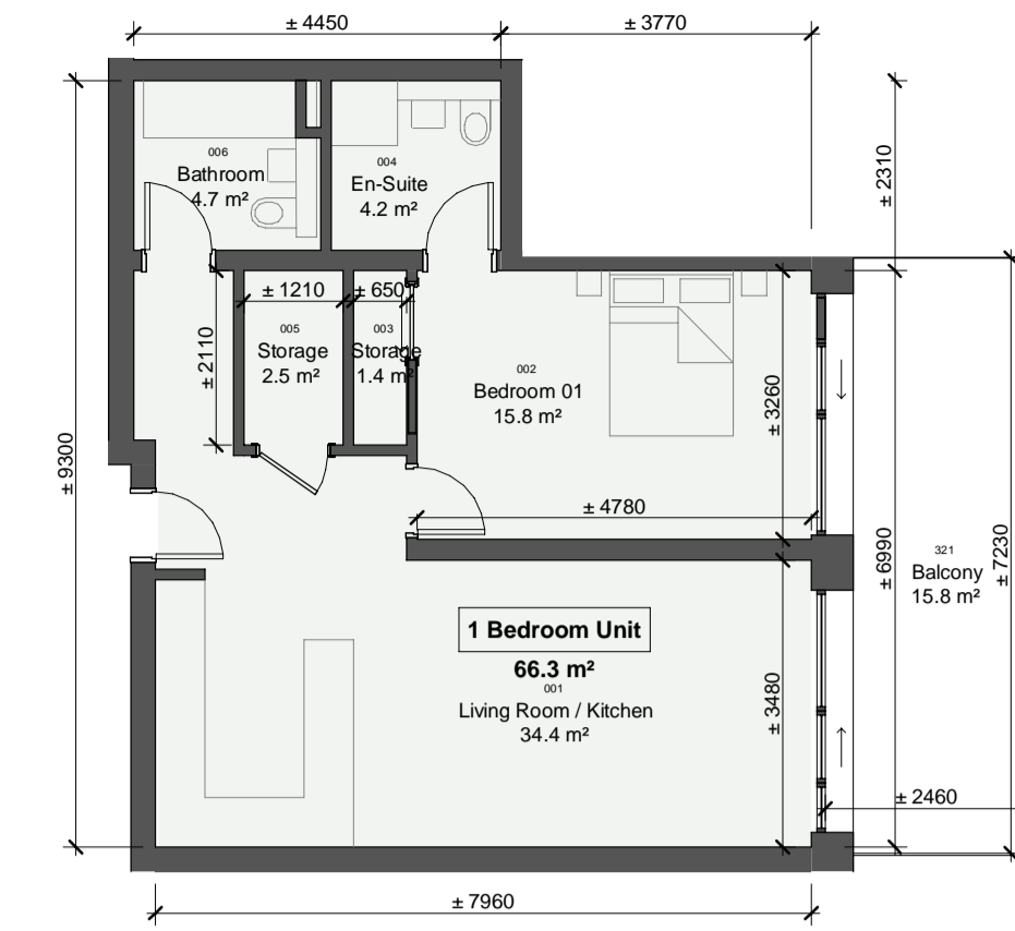
3 Unit Type 1BR-B-1 scale 1 : 100
