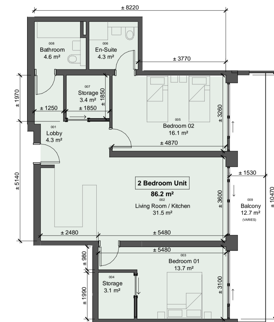
10 Unit Type 2BR-D-1 scale 1 : 100
